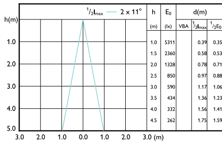
LEDspot_90W_E27_PAR38_827_25°
