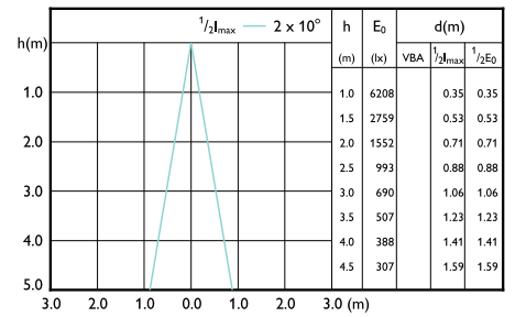
14-120W E27 PAR38 25D 830 3000K
