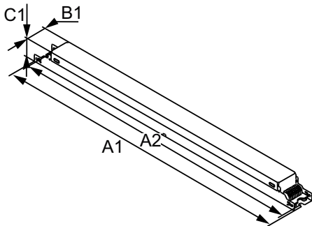
ELE DIMMING BALLAST (1) F54T5/HO 277V
