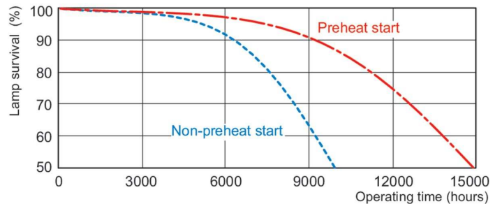
Life Expectancy Diagram - PL-Q 38W/827/4P 1CT/10BOX
