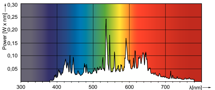
Spectral Power Distribution Colour - MASTERC CDM-TC Elite 50W/942 G8.5 ICT
