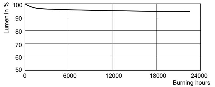
Lumen Maintenance Diagram - MASTER SOX-E 91W BY22d 1SL/12
