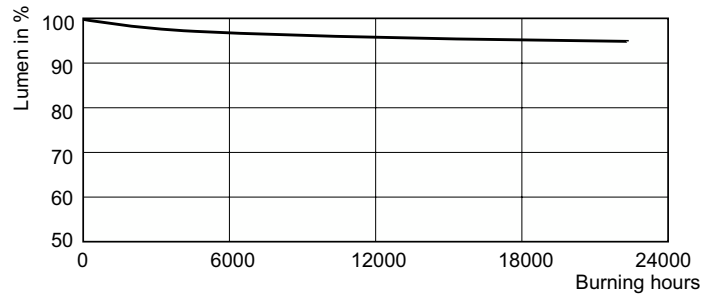
Lumen Maintenance Diagram - SOX 135W BY22d 1SL/12
