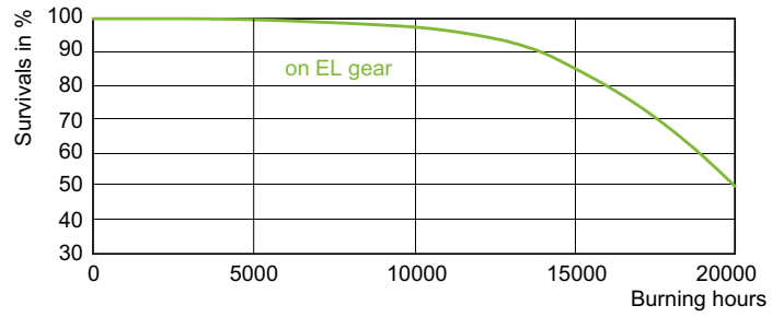
Life Expectancy Diagram - MASTER colour CDM-TC Elite 50W/930 G8.5 1CT/12
