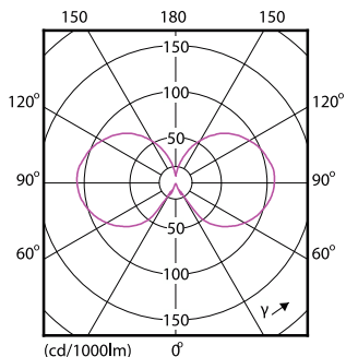
Light Distribution Diagram - CLA LEDLuster ND 4-40W P45 E14 827 CL
