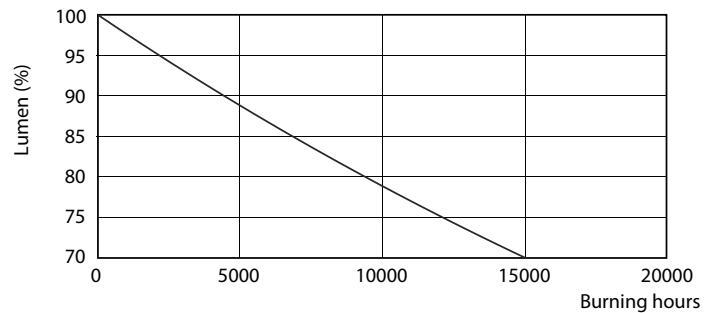
Lumen Maintenance Diagram - CorePro LEDbulb ND 5-40W A60 E27 830
