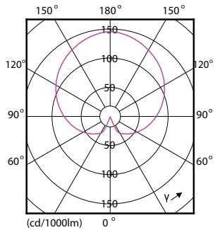
Light Distribution Diagram - MAS LED bulb DT 9-60W E27 927-922 A60 FR
