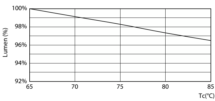
Lumen Maintenance Diagram - MAS LEDtube VLE 1500mm HO 20.5W 830 T8
