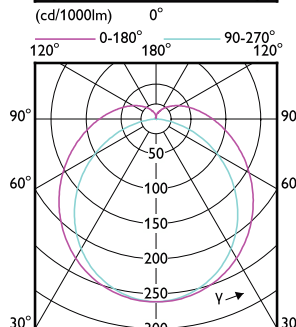
(cd/1000lm) 0° 0-180° 90-270°
