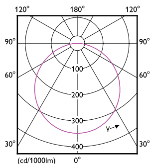
Light Distribution Diagram - DN027B LED9/NW L125 SQ
