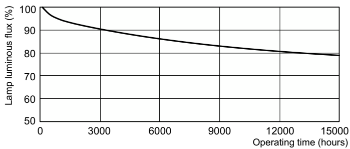
Lumen Maintenance Diagram - PL-T 18W/830/A/4P 1CT/5X10BOX ALTO
