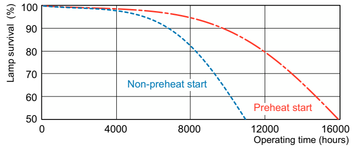
Life Expectancy Diagram - MASTER TL5 Circular 40W/865 1CT/10
