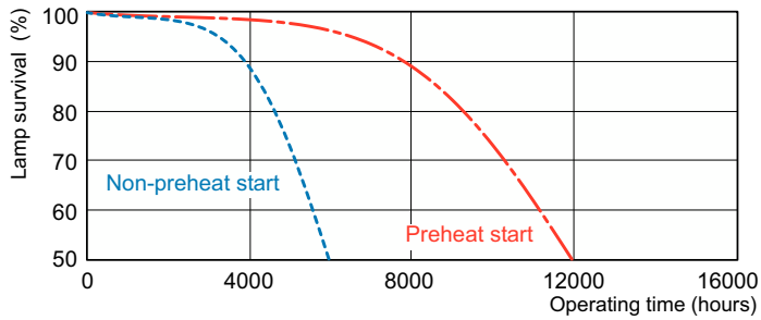
Life Expectancy Diagram - MASTER TL5 Circular 40W/865 1CT/10
