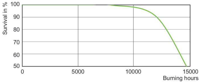
Life Expectancy Diagram - MST CosmoWh CPO-TW 90W/840 PGZ12 1CT
