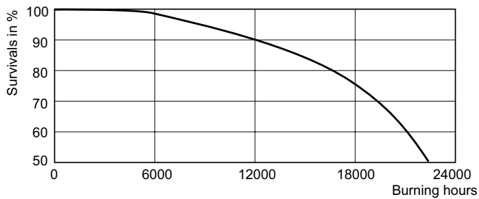
Life Expectancy Diagram - MASTER SOX-E 66W BY22d 1SL/12
