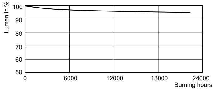
Lumen Maintenance Diagram - SOX 55W BY22d 1SL
