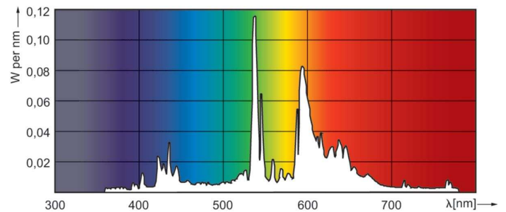
Spectral Power Distribution Colour - CDM20/TC/830 Elite
