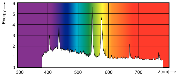
Spectral Power Distribution Colour - MSR Gold 1500/2 FastFit
