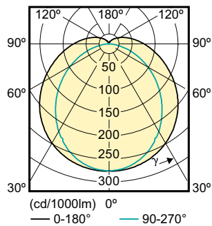
Light Distribution Diagram - MAS LEDtube 1500mm SO 20W 840 T8
