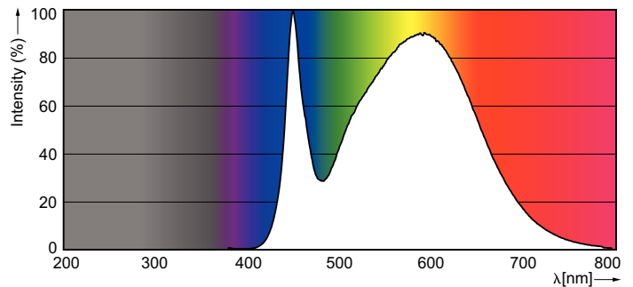
Spectral Power Distribution Colour - MAS LEDtube STD 1200mm 14.5W840 T8 I
