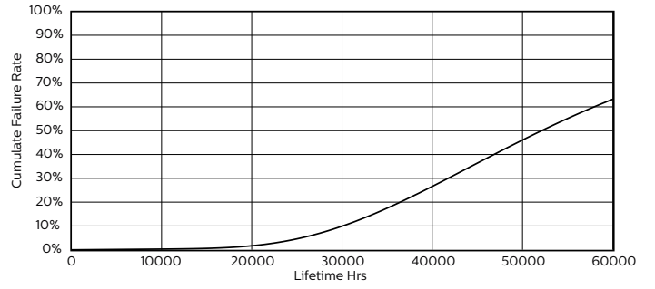
Life Expectancy Diagram - 10T8/48-4000 IF 10/1 TAA/NAFTA
