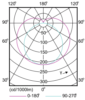
Light Distribution Diagram - 10T8/48-5000 IF 10/1 TAA/NAFTA
