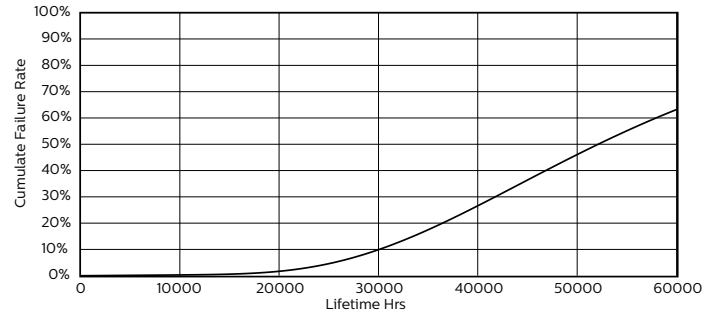
Life Expectancy Diagram - 10T8/48-5000 IF 10/1 TAA/NAFTA
