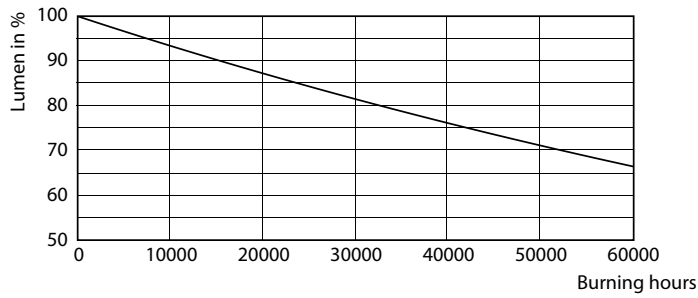
Lumen Maintenance Diagram - 10T8/48-5000 IF 10/1 TAA/NAFTA
