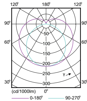
Light Distribution Diagram - 14T8/48-3500 IF 10/1 DIM TAA/NAFTA
