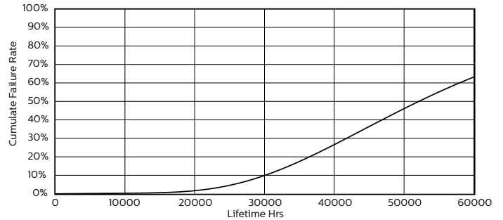
Life Expectancy Diagram - 14T8/48-3500 IF 10/1 DIM TAA/NAFTA
