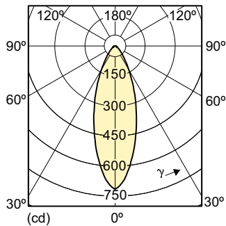
Light Distribution Diagram - CorePro LEDspotMV 5-50W GU10 840 36D
