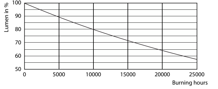
Lumen Maintenance Diagram - Essential LED 4.6-50W GU10 827 36D
