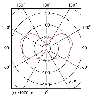
Light Distribution Diagram - CLA LEDBulb D 7-50W ST64 E27 820 GOLD
