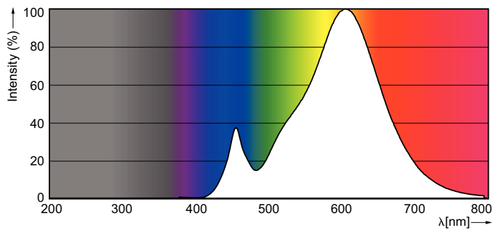
Spectral Power Distribution Colour - LEDClassic 4-50W A60 E27 WW CL ND APR
