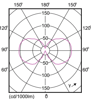
Light Distribution Diagram - LEDClassic 4-50W A60 E27 WW CL ND APR
