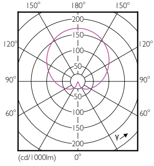
Light Distribution Diagram - CorePro LED bulb ND 5-40W A60 E27 865
