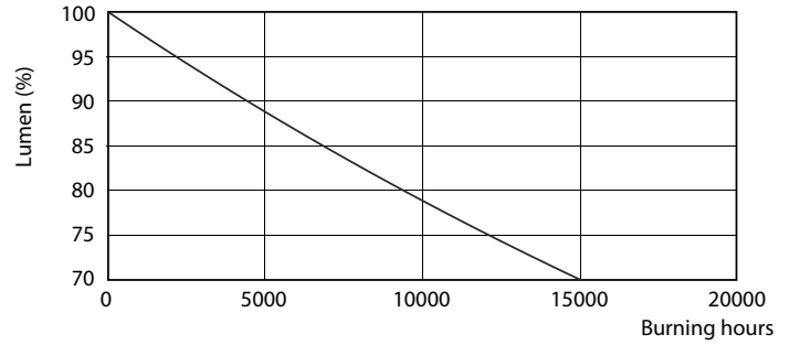
Lumen Maintenance Diagram - CorePro LED bulb ND 5-40W A60 E27 865
