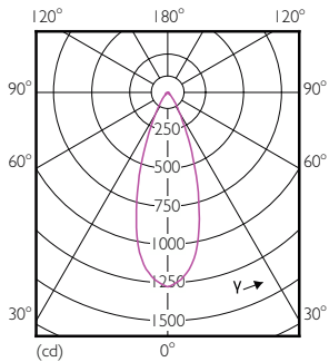
Light Distribution Diagram - MAS LEDspot CLA D 6-50W 840 PAR20 40D
