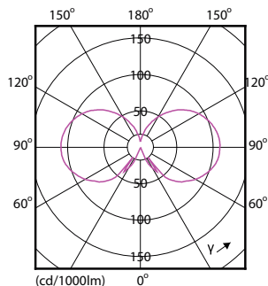
Light Distribution Diagram - CLA LEDCandle D 5-40W B35 E14 827 CL
