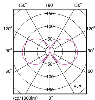
Light Distribution Diagram - CLA LEDLuster D 2.7-25W P45 E14 827 CL
