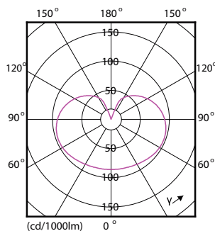
Light Distribution Diagram - LED SSW 100W A67 E27 WW-CW FR ND 1BC/6
