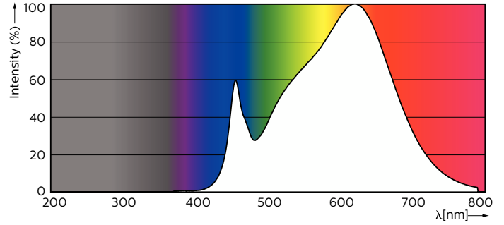
Accent Lighting Spots - MAS LED spot VLE D 4.9-50W GU10 930 60D Spectral Power Distribution Colour - MAS LED spot VLE D 4.9-50W GU10 930 60D
