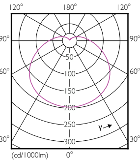
Light Distribution Diagram - LEDBulb 14.5W E27 6500K 230V A67 APR
