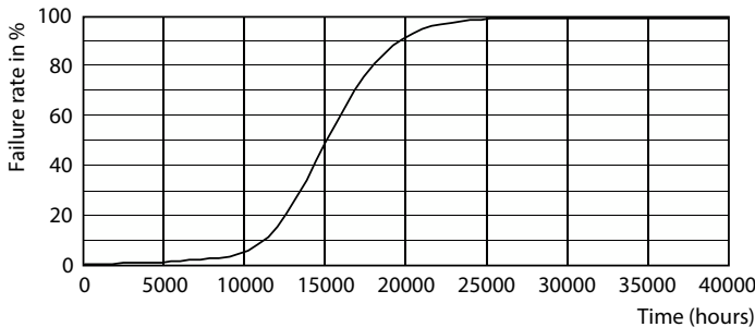
Life Expectancy Diagram - 9A19/PER/850/P/E26/DIM 8/1FB
