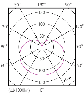
Light Distribution Diagram - 9A19/PER/850/P/E26/DIM 8/1FB
