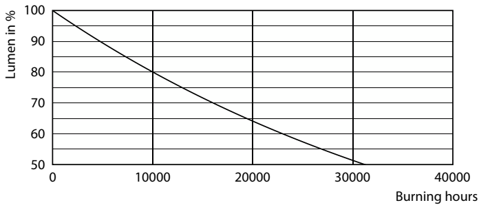
Lumen Maintenance Diagram - 8A19/LED/830/ND 120V E27 1BC MX
