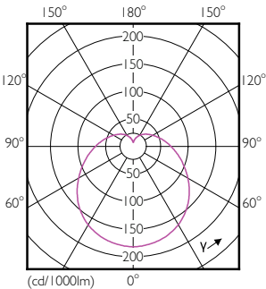
Light Distribution Diagram - 8A19/LED/830/ND 120V E27 1BC MX
