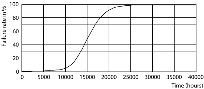
Life Expectancy Diagram - 8A19/LED/830/ND 120V E27 1BC MX
