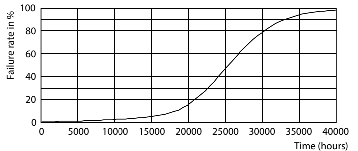
Life Expectancy Diagram - MASLEDBulb DT 15-100WE27 927-922 A67FR
