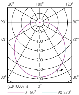
Light Distribution Diagram - TForce HB 100-85W E40 865 120D LA
