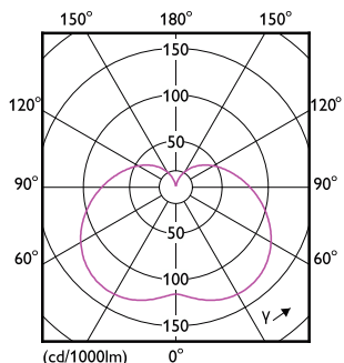
Light Distribution Diagram - TForce Core HB MV ND 37-35W E27 830
