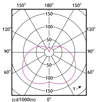
Light Distribution Diagram - TForce Core HB MV ND 40-35W E27 840
