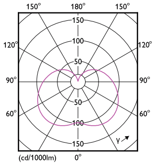
Light Distribution Diagram - TForce Core HB MV ND 48-42W E27 830
