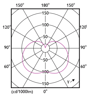
Light Distribution Diagram - TForce Core HB MV ND 50-42W E27 840
