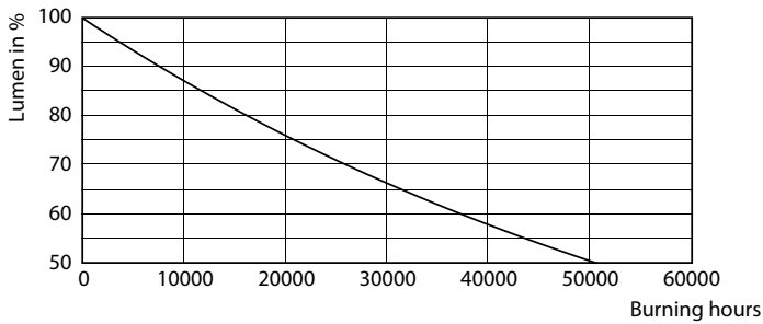
Lumen Maintenance Diagram - LEDBulb 23W E27 6500K W A30 1PF/6 MX
