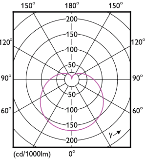
Light Distribution Diagram - LEDBulb 23W E27 6500K W A30 1PF/6 MX
