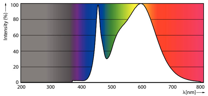
Spectral Power Distribution Colour - 145HB/LED/840/ND WB UDL BB 4/1
