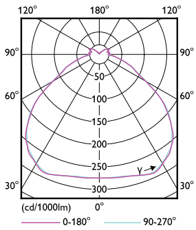
Light Distribution Diagram - 145HB/LED/840/ND WB UDL BB 4/1
