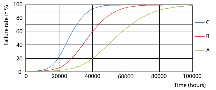
Life Expectancy Diagram - 12.5T8/COR/48-830/MF17/G 10/1
