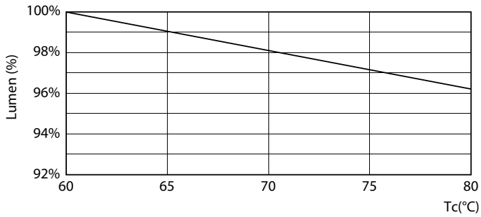
Lumen Maintenance Diagram - 12.5T8/COR/48-830/MF17/G 10/1
