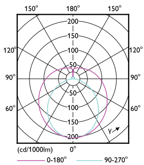
Light Distribution Diagram - 12.5T8/COR/48-830/MF17/G 10/1
