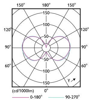
Light Distribution Diagram - 63CC/LED/850/ND EX39 G2 BB 6/1
