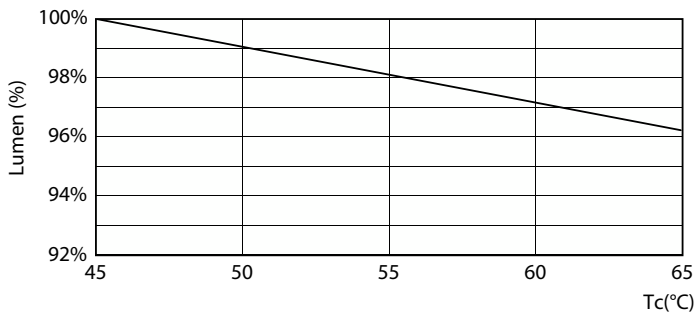
Lumen Maintenance Diagram - 16.9T8/MAS/48-840/MF25/P 10/1
