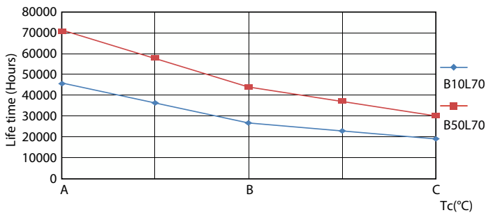
Life Expectancy Diagram - 16.9T8/MAS/48-840/MF25/P 10/1
