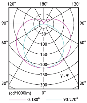
Light Distribution Diagram - 16.9T8/MAS/48-840/MF25/P 10/1
