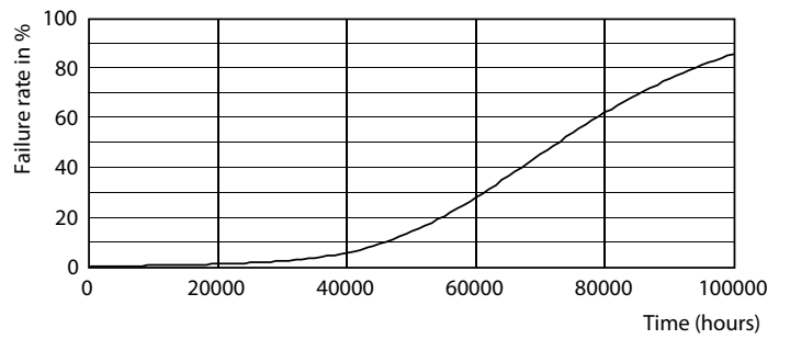
Life Expectancy Diagram - 16.9T8/MAS/48-850/MF25/P 10/1
