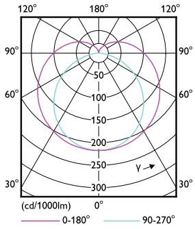
Light Distribution Diagram - 16.9T8/MAS/48-850/MF25/P 10/1
